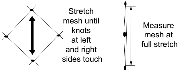
Figure 2-1 How to measure net mesh
